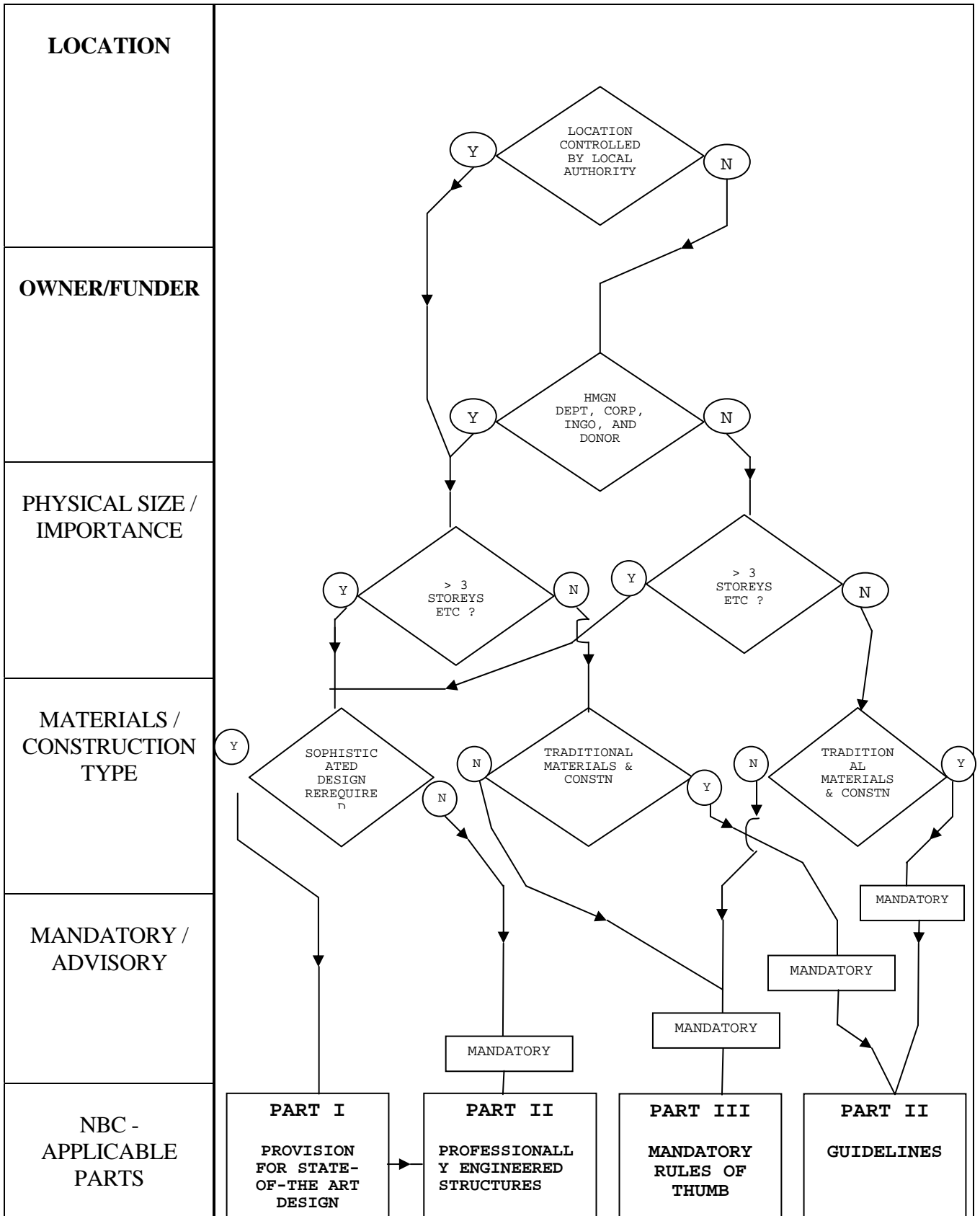
Figure 1: Flow Chart Showing Minimum Design Requirements
